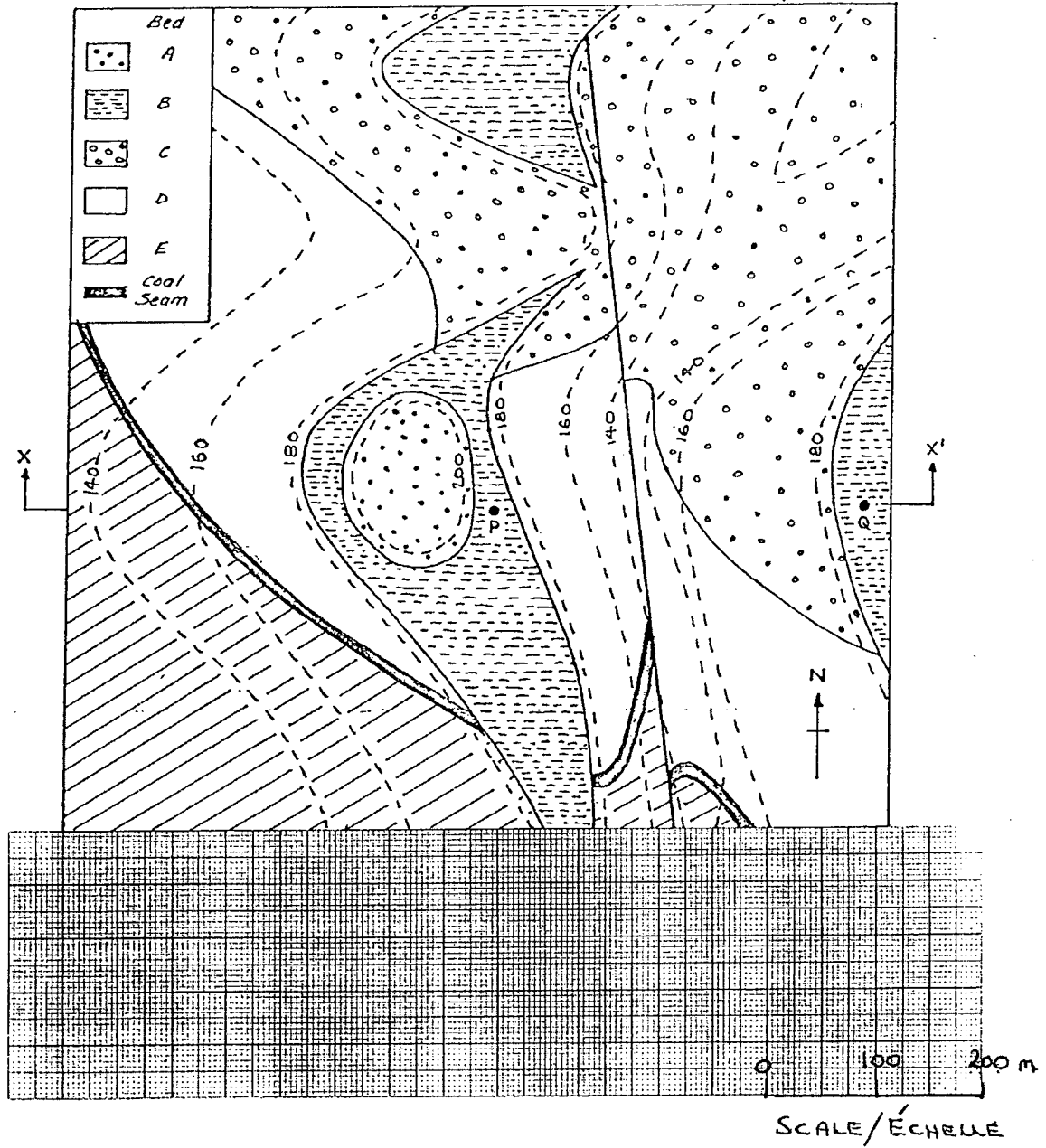
Figure Q1. Contours (m)
