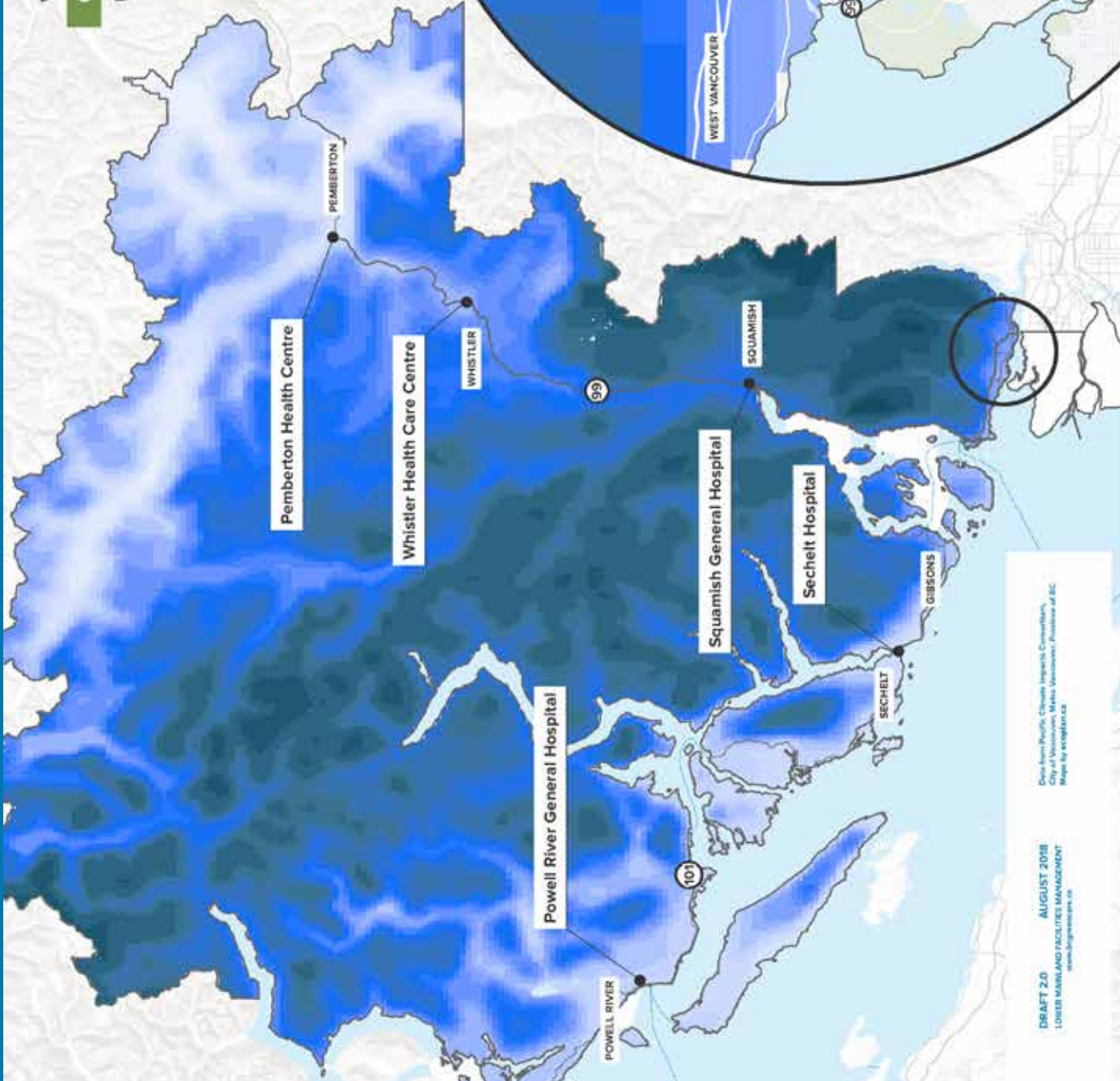
R95P Wettest Day Precipitation - Future (2050)
