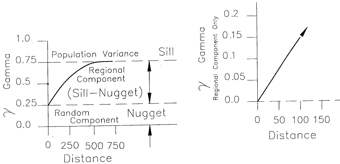
Figure 4.3 Variogram model
