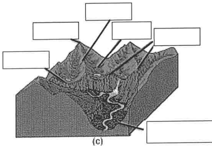
Figure Q3-2 – Fill in the six blanks above indicating the glacial features
